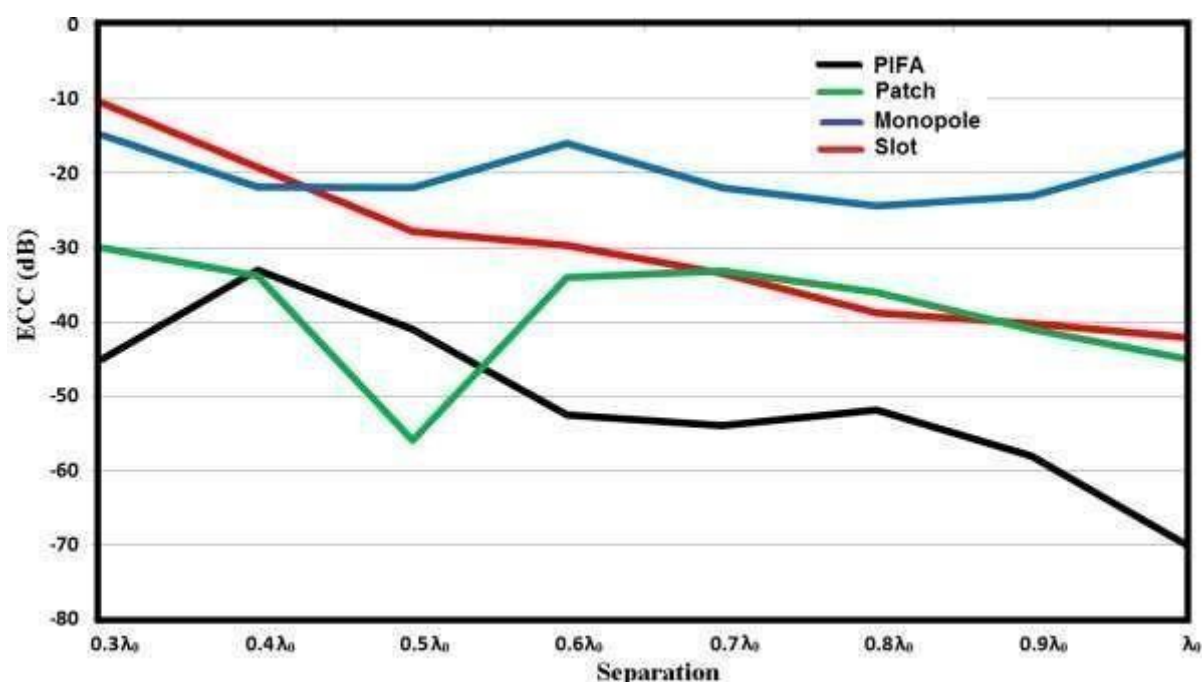
Figure 1: Comparison of envelope correlation coefficient (ECC) with different antennas types at varying separation (in terms of \lambda_0 )
